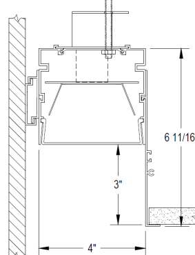
GPD4 4" Housing Width Regress 0", 1", 2", 3"
