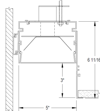
GPD5 5" Housing Width Regress 0", 1", 2", 3"
