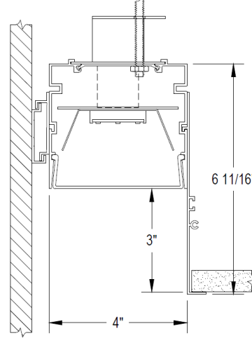
GPD4 4" Housing Width Regress 0", 1", 2", 3"
