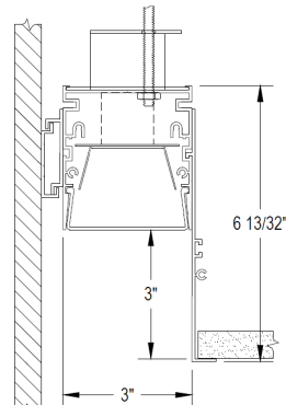
GPD3 3" Housing Width Regress 0", 1", 2", 3"
