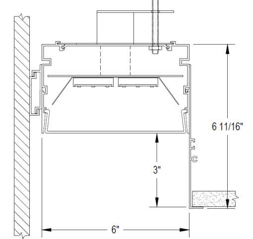
GPD6 6" Housing Width Regress 0", 1", 2", 3"
