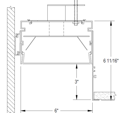
GPD6 6" Housing Width Regress 0", 1", 2", 3"
