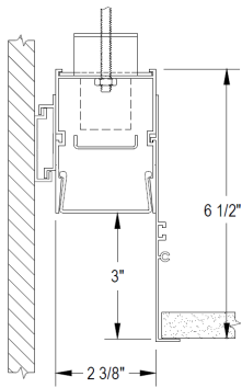
GPD2 2.4" Housing Width Regress 0", 1", 2", 3"
