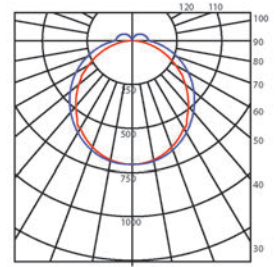
Totally Asymmetric Solid: 180-0 Degrees Dashed: 270-90 Degrees
