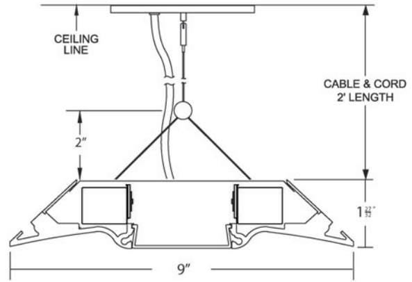
Inverted Y Cable Mount: Specify Y code in catalog #
