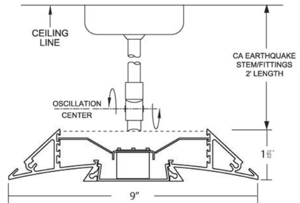
CA Earthquake Stem Mount: Specify SEQ code in catalog #
