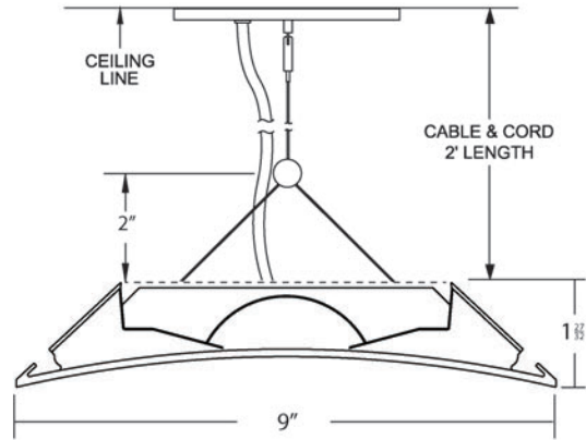
Inverted Y Cable Mount: Specify Y code in catalog #
