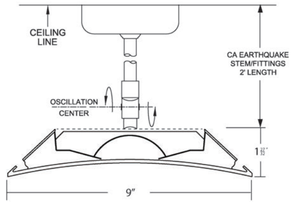
CA Earthquake Stem Mount: Specify SEQ code in catalog #
