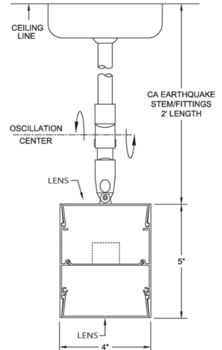
CA Earthquake Stem Mount: Specify SEQ code in catalog #
