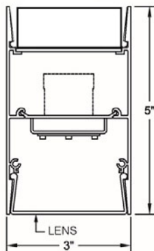
LED LAMPING
