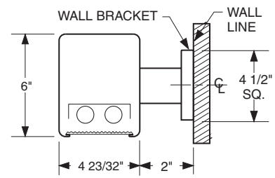
Wall Bracket (Specify WB)
