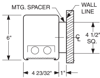
Wall Hung (Specify WHM)
